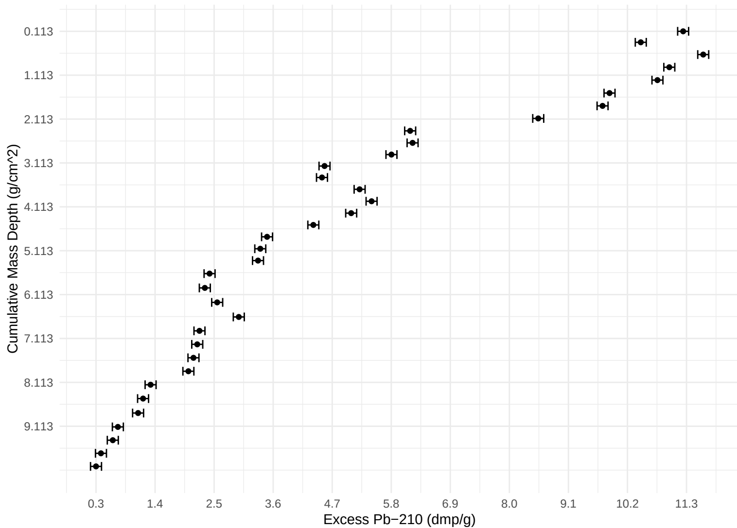
Excess Pb-210 vs Cumulative Mass Depth
